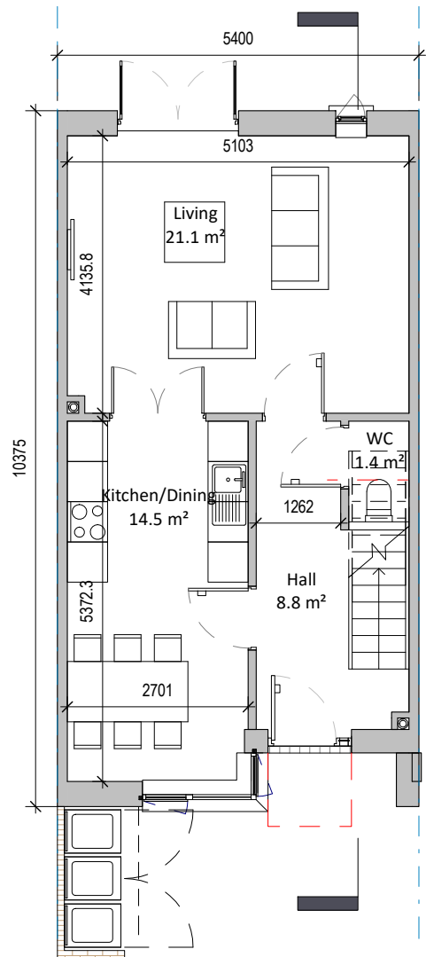
① Type 2 Level 00 1:100
