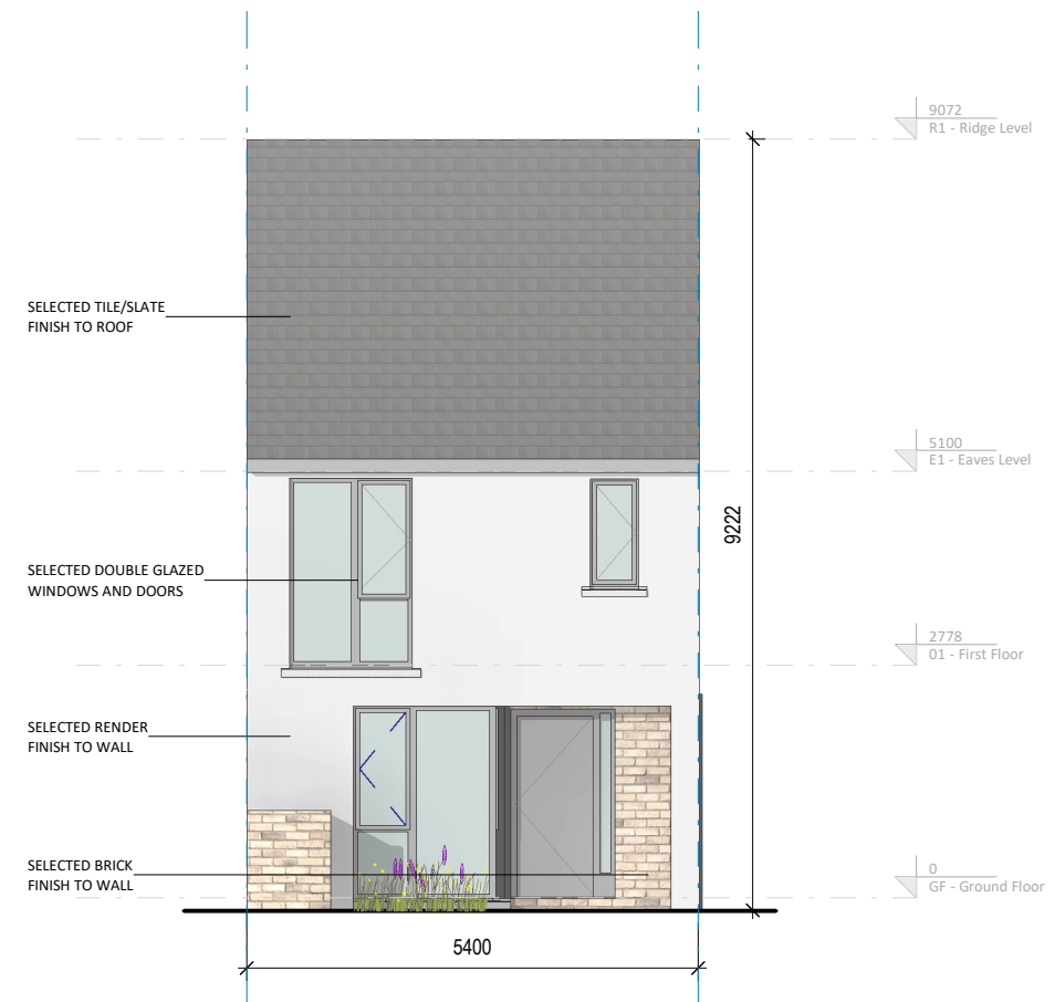
③ Type 2 Front Elevation 1:100
