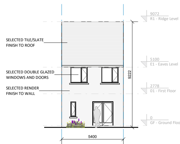
④ Type 2 Rear Elevation 1:200
