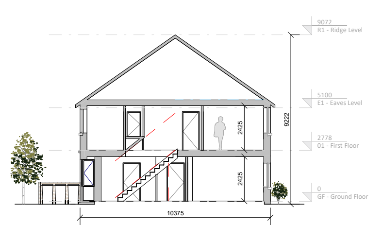
⑤ Type 2 Section 1:200
